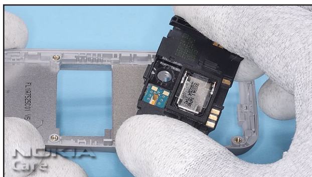
22. The MECHANICAL ANTENNA ASSEMBLY can be lifted up now.
