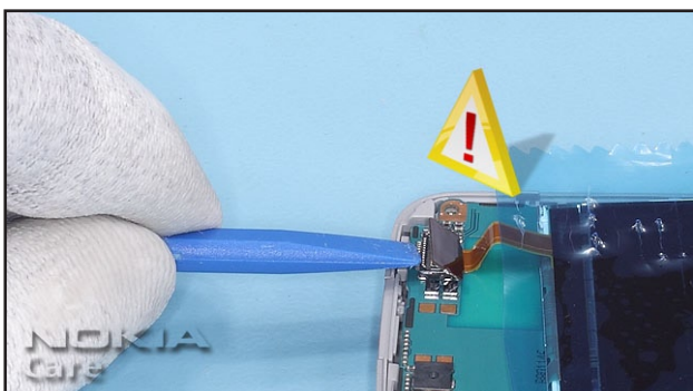
11. Be double carefully while opening the flex foil connector of the LCD. Remove the LCD now.
