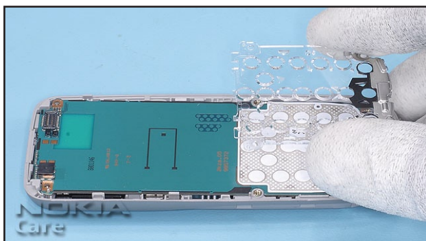
12. Lift up the LIGHT GUIDE ASSMBLY.
