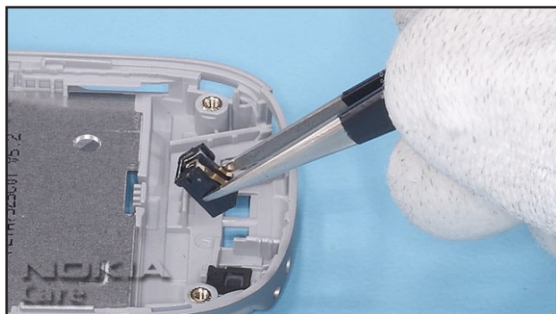
18. ...remove it with tweezers.
