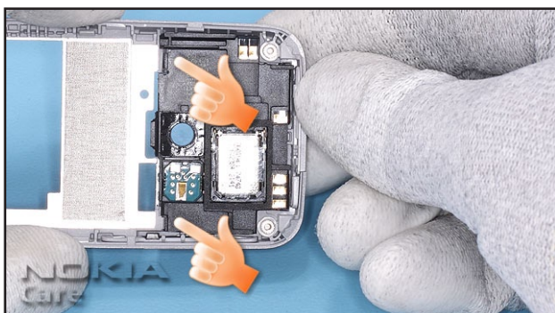
19. The MECHANICAL ANTENNA ASSEMBLY is fixed with 2 plastic clips.
