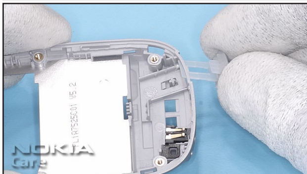
16. Remove the USB DOOR.
