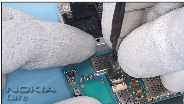
15. Use the C-COVER as support while removing the CAMERA MODULE.
