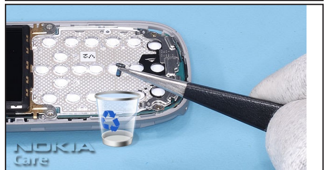
8. Discard these screws. Do not use them again.
