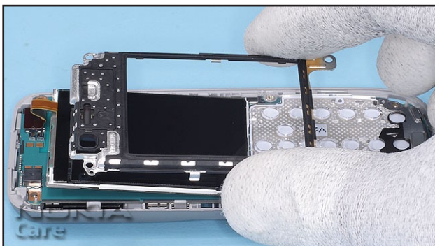
9. Lift up the LCD SHIELD.
