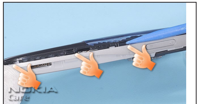
4. Unlock these 3 clips on both sides with the SS-93.
