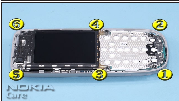
7. Unscrew these 6 Torx Plus size 6 screws in the order shown.
