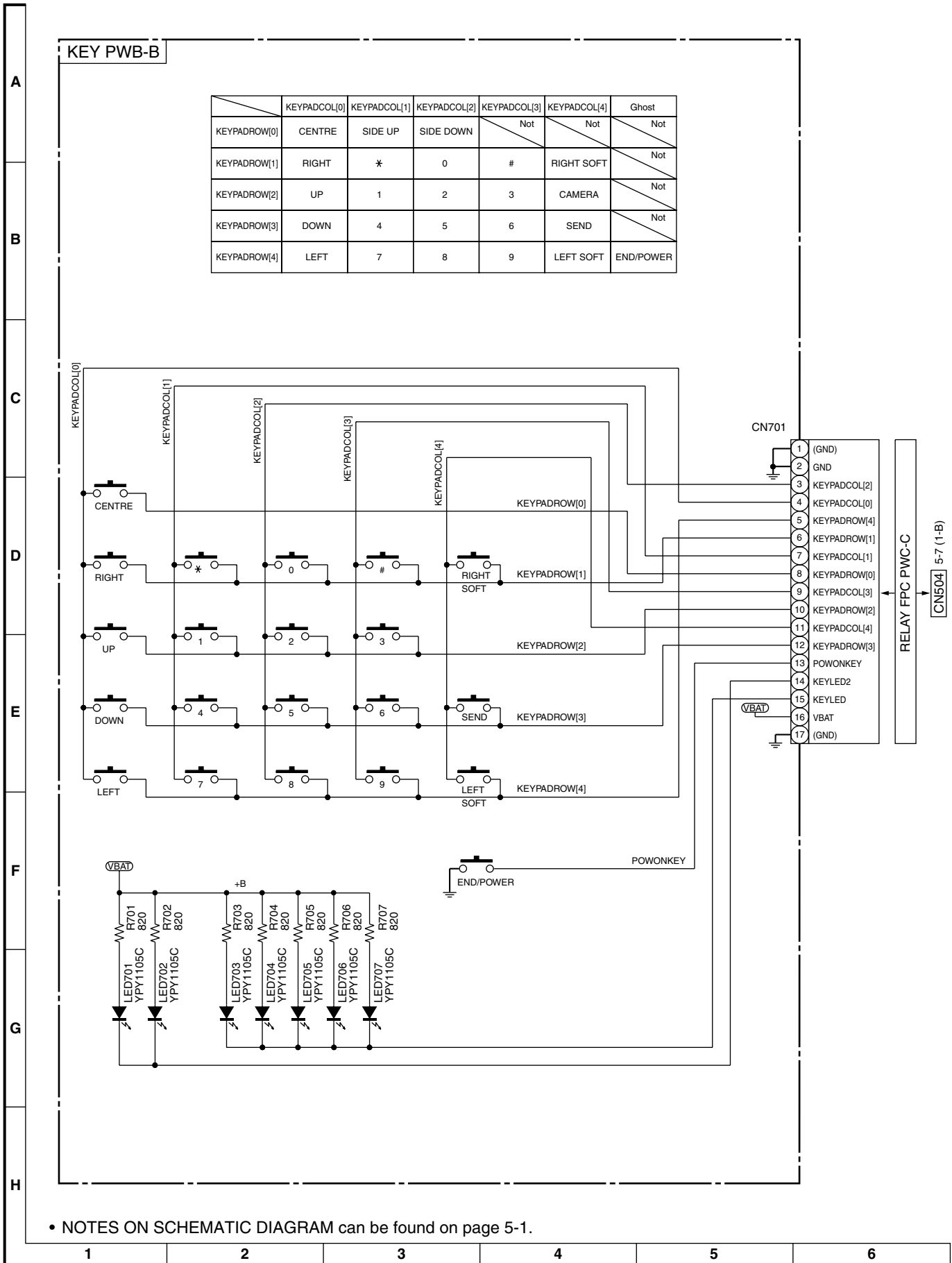
Figure 8 SCHEMATIC DIAGRAM (6/6)
