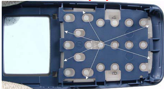
7.) Fit the Keymat to the A-Cover , paying attention to its correct position.
