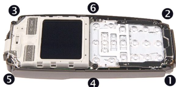
8.) Unscrew the six, Torx Plus® size 6 screws in the shown order. For assembly, use the reverse order and a Torx Plus® size 6 driver with a torque setting of 24Ncm.
