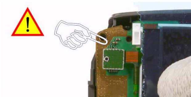
13.) Take care to the surrounding components when opening the LCD connector.
