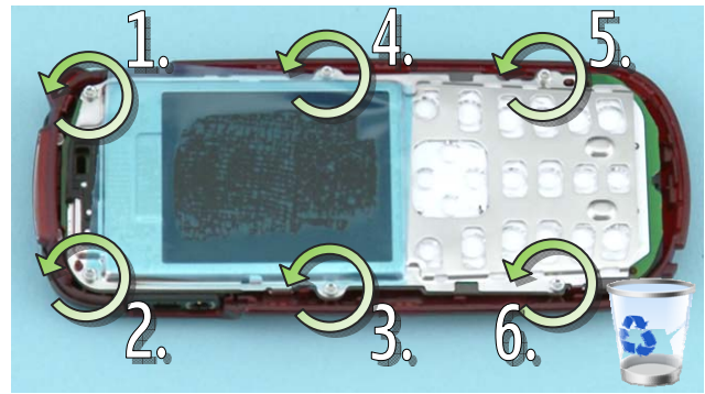
8) Unscrew the six Torx+ 4 screws in the order shown.
