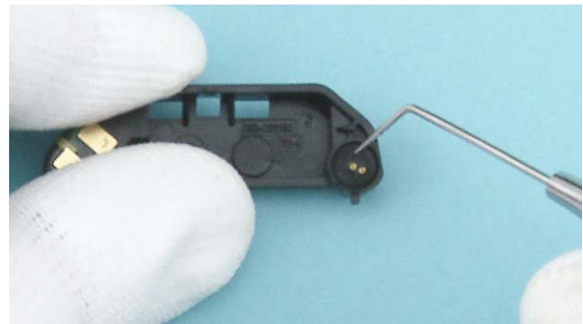
12) Use the dental tool to remove the MICROPHONE.
