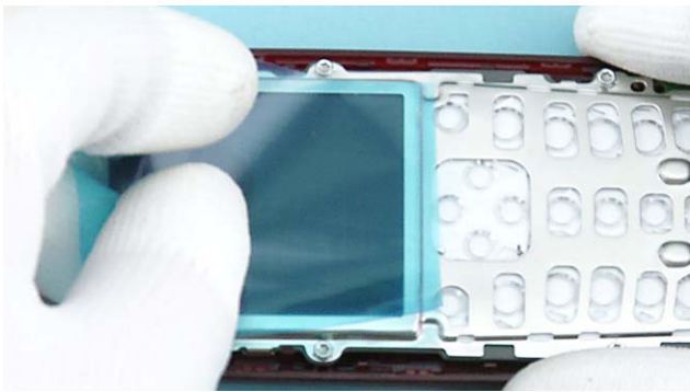
7) Protect the LCD with a protective film.
