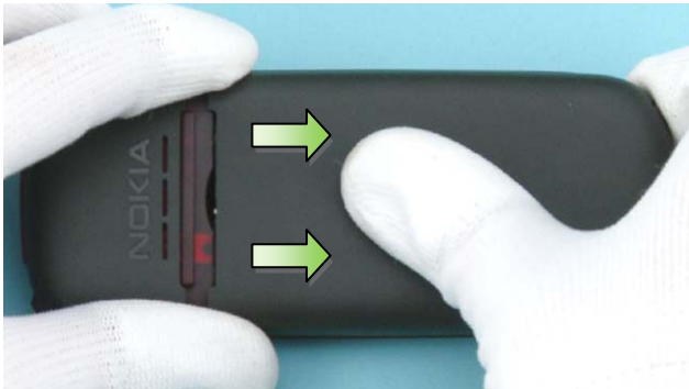
3) To remove the B-COVER pull it in the direction shown.
