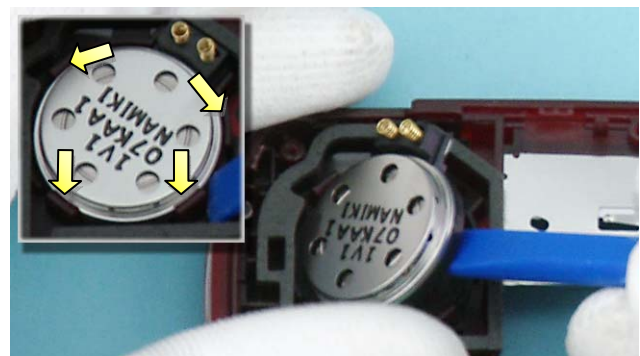
10) Release the clips holding the EARPIECE/IHF SPEAKER/VIBRATOR with the SS-93. Then remove the assembly.
