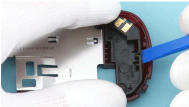
11) To release the ANTENNA ASSEMBLY first insert the SS-93 between the assembly and the D-COVER. Then gently lift the assembly up.
