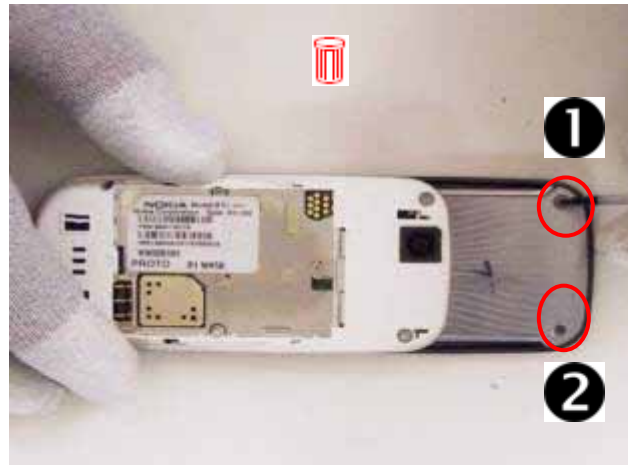
4) Use the #4 TORX screwdriver to remove the 2 screws in the order shown. Discard the screws.
