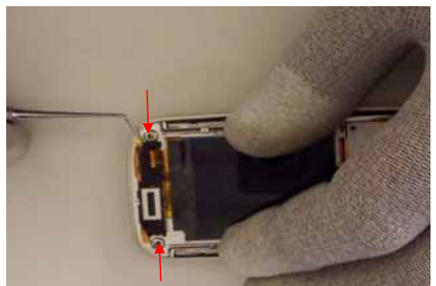
10) Use the dental pick to release the earpiece holder assy. Repeat on the opposite side.
