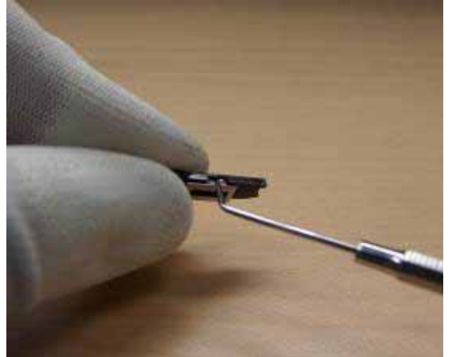
12) Use the dental pick to release the earpiece from the frame.
