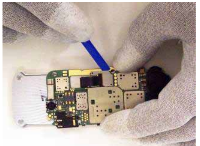
20) Use the SS-93 tool to release the UI Flex connector from the engine side.
