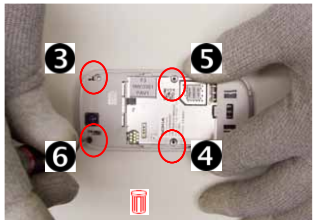
8) Use the #6 TORX screwdriver to remove the 4 screws in the order shown. Discard the screws.
