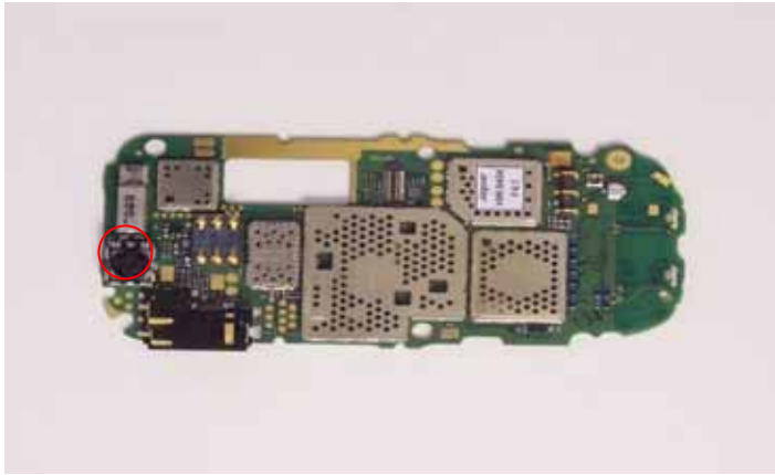
27) Use the SS-88 camera tool to remove the camera module.
