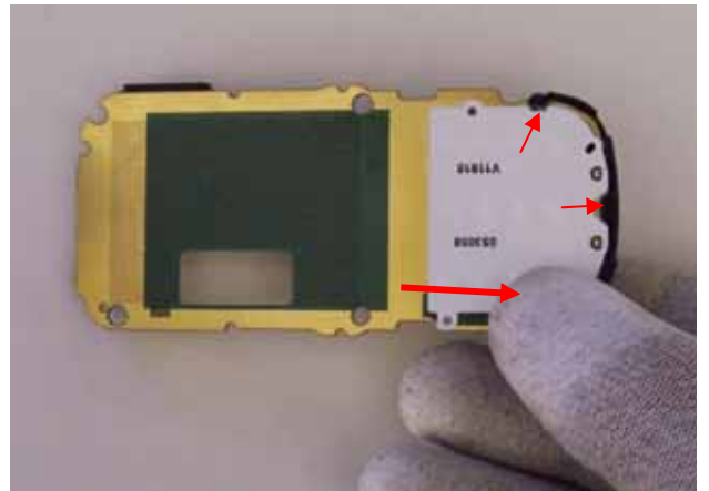
24) Push down the tab with thumb and then pull down to release the other tabs.
