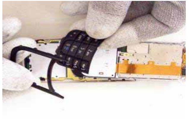
18) Lift and remove the numerical keymat and C-Cover Assy.
