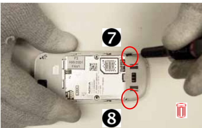
9) Use the #4 TORX screwdriver to remove the 2 screws. Discard the screws.
