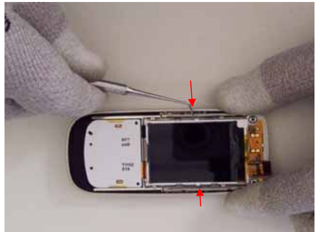
14) Insert the dental pick in the center to release the LCD tabs.
