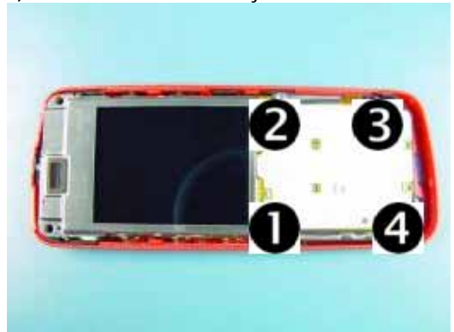
6.1) Screw order
