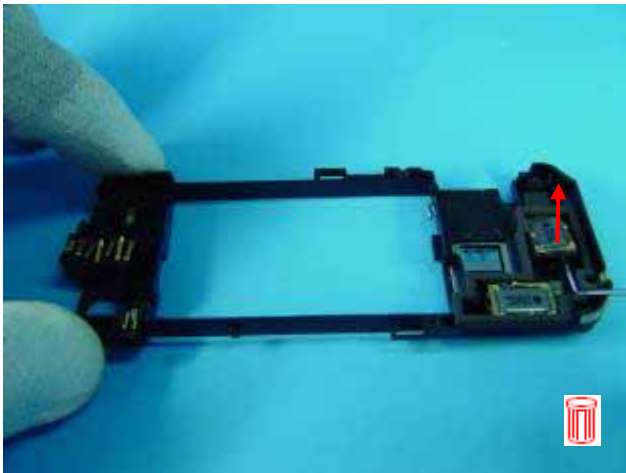
9) Use a dental tool to release the IHF SPEAKERS. IHF SPEAKERS has always to be renewed. DC-Jack and AV CONNECTOR can remove easily.
