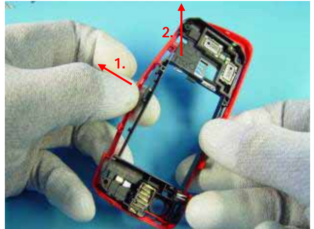
8) Release the B-COVER SUB ASSY from the MIDBAND ASSY as shown.
