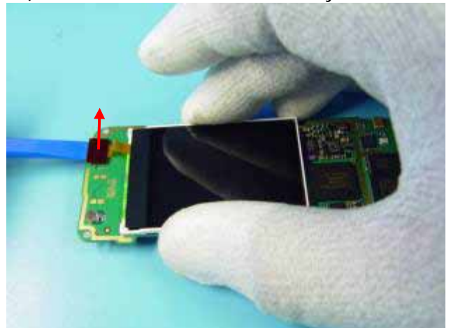
14) Disconnect the DISPLAY and take it away.
