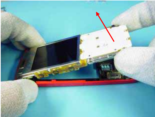
7) Separate the UI SHIELD ASSY inclusive DISPLAY and PWB from the B-COVER SUB ASSY.
