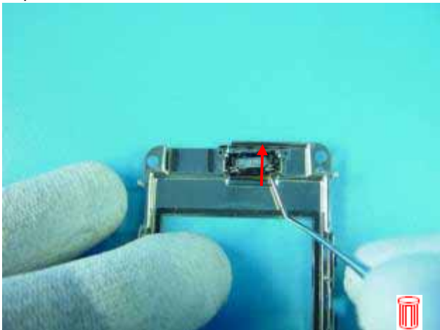
13) Lift up the EARPIECE with dental tool.
