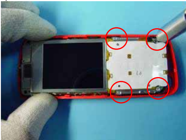
6) Use T6+ to remove the screws.
