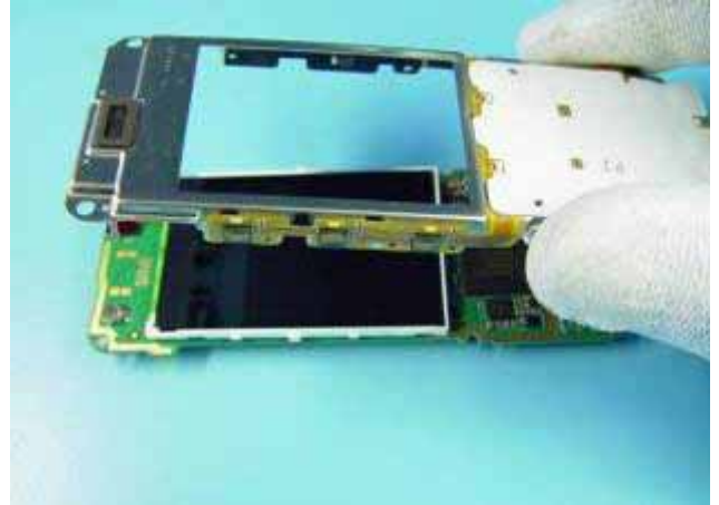
12) UI SHIELD ASSY can be taken away.
