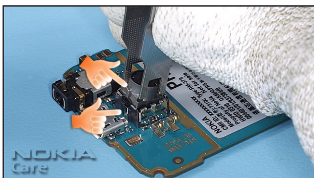
20. Use the SS-8 to remove the Camera Module.
