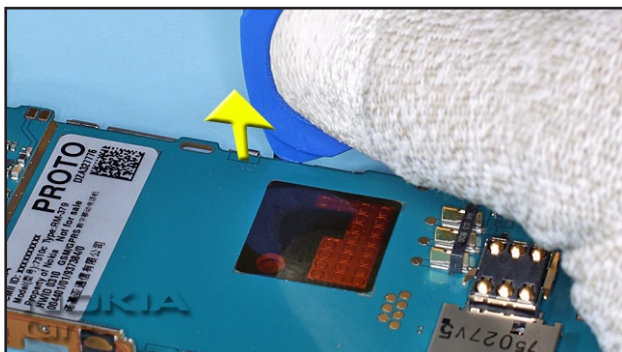
17. Unlock the PWB with the SRT-6.
