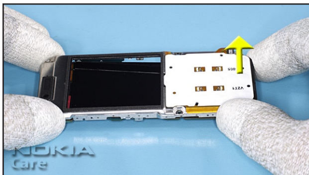
18. Remove the UI Assy.
