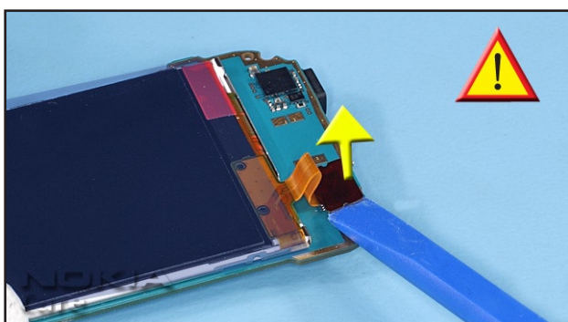
19. Carefully open the LCD connector.
