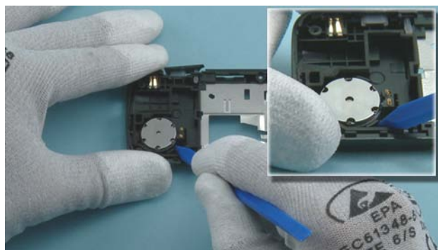
20) Use the sharp end of the SS-93 to release the EARPIECE / SPEAKER / VIBRA.
