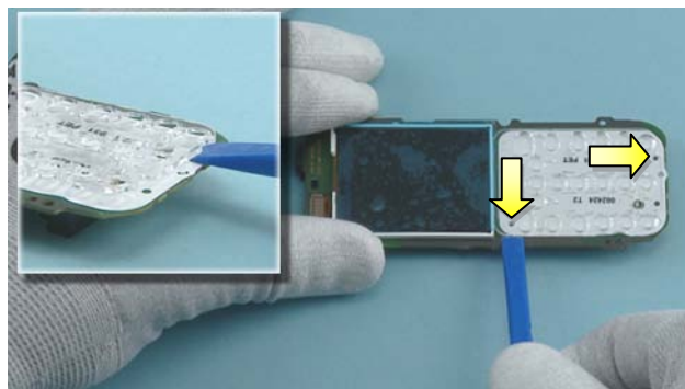
28) Release the two guiding pins holding the LIGHT GUIDE with the SS-93.
