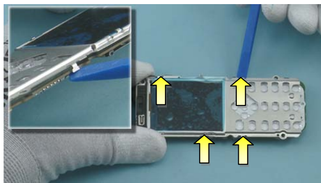
26) Release the four clips holding the UI SHIELDING with the SS-93.
