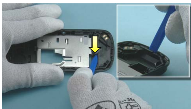
24) Use the sharp end of the SS-93 to release the ANTENNA MODULE clip and then use the flat end of the SS-93 to release the bottom end of the ANTENNA MODULE.
