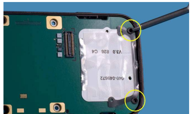
12) Unscrew the two TORX 6+ screws.
