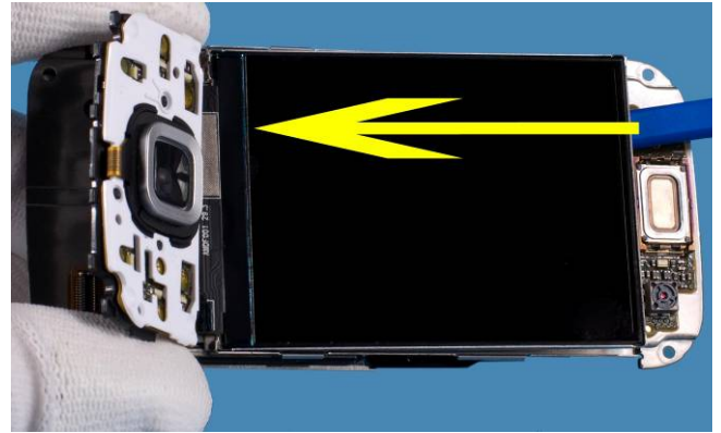
38) Use SS-93 tool to release LCD.
