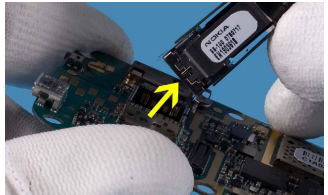
16) Remove the CAMERA with SS-100 tool.
