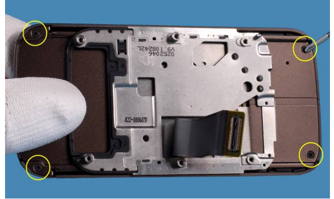
32) Unscrew the four crosshead screws.
