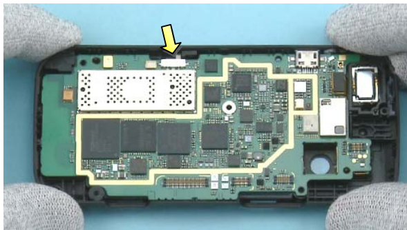
3) After assembling engine board into the B-COVER, check the right alignment of the LOCK KEY SWITCH.
