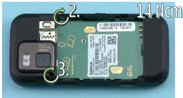
7) Tighten these two M1.4x3.6 TORX PLUS 4IP screws to the torque of 14 Ncm in the order shown.
