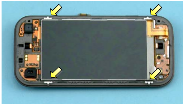
1) Before placing the A-COVER make sure all the four A-BEZEL GROUND CLIPS are in place.
