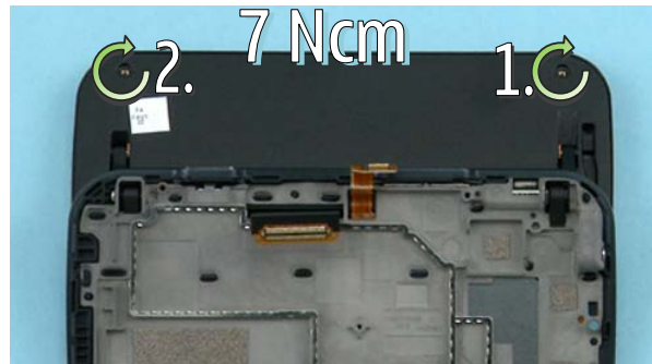
4) Tighten the two M1.2X2, PANHEAD 2.5X0.6 T PLUS-4IP screws to the torque of 7 Ncm in the order shown.
