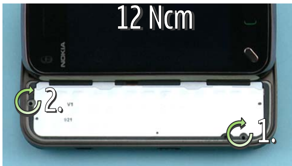
5) Tighten the two M1.4 x 5.8 P3642 screws to the torque of 12 Ncm in the order shown.
