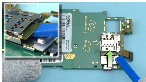
24) Detach one end of the READER FPC using the SS-93.
