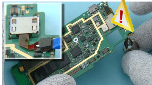
22) Disconnect the camera connector from the engine board with the SS-93. Be careful not to damage the components nearby! Remove the camera.
