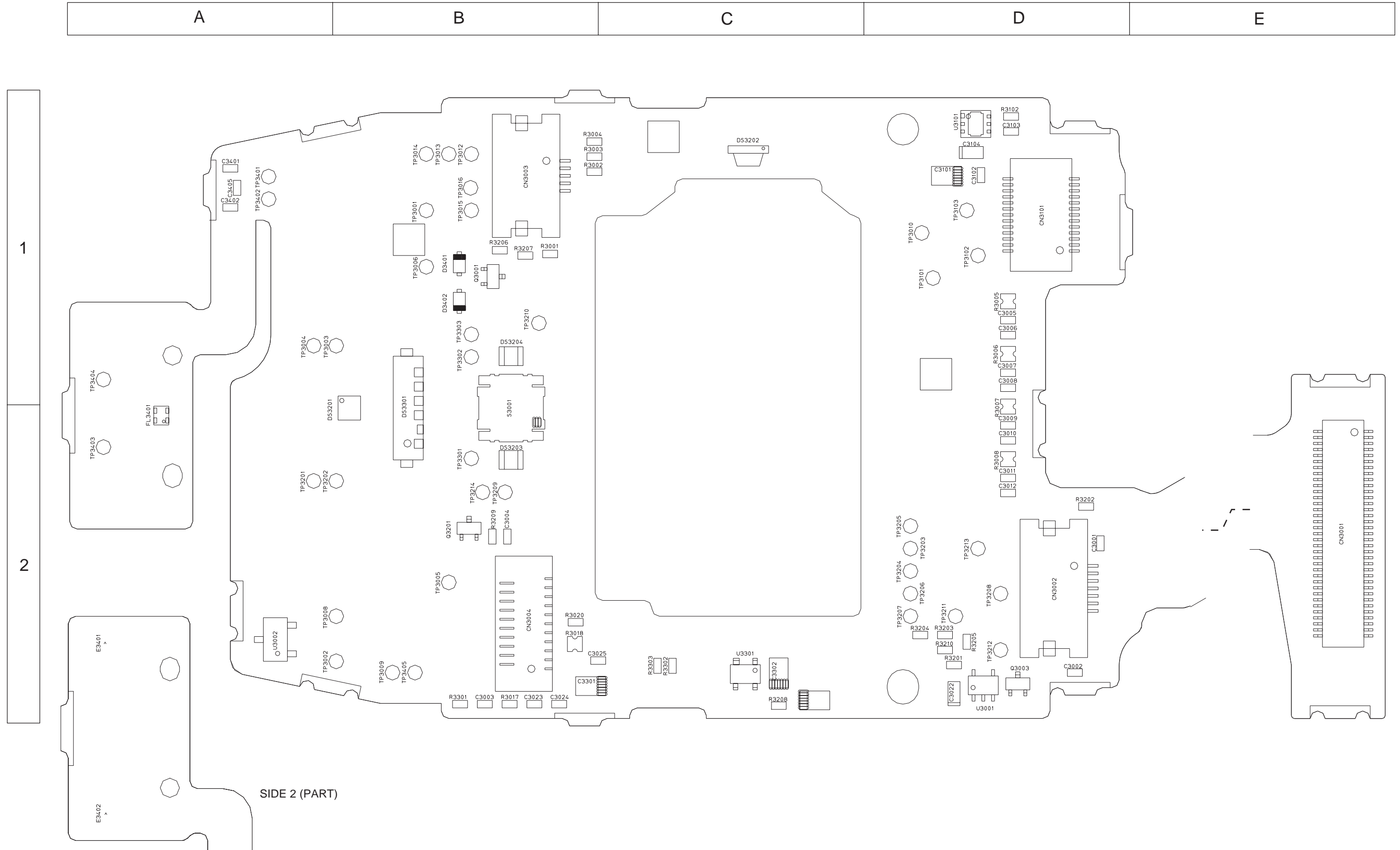
Figure 11.3: Display PCB Layout
